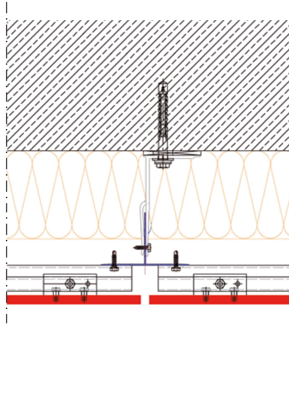
JOINT VERTICAL
